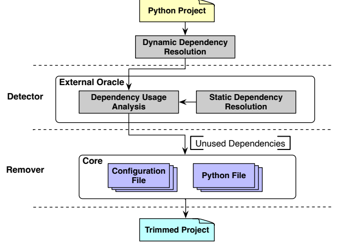
Fig. 3: High-level architecture of PYTRIM.
